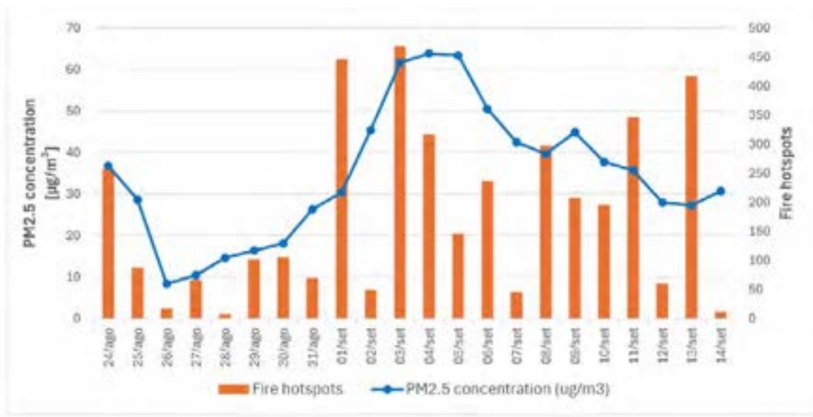
Figure 4. Daily fire hotspots in Minas Gerais and PM2.5 concentration.
