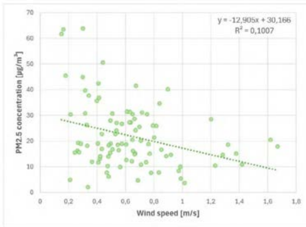
Figure 8. PM2.5 concentration versus wind speed.
