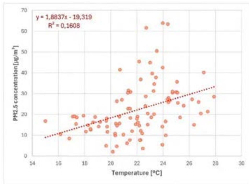
Figure 7. PM2.5 concentration versus temperature.
